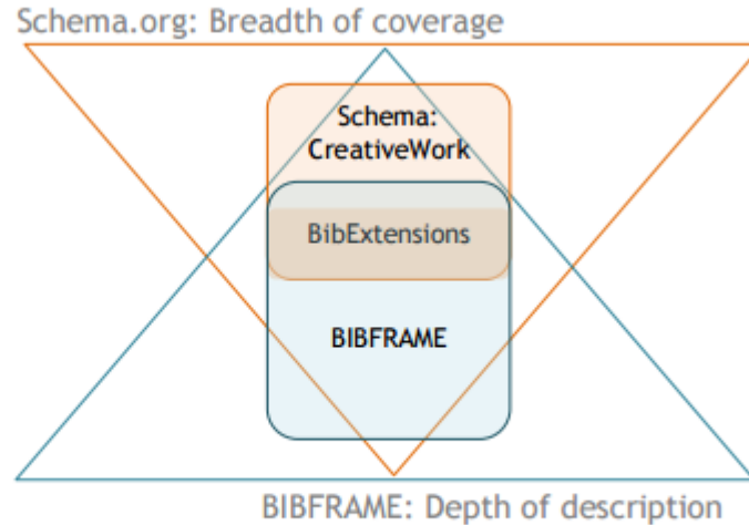
Figure 4.1. High-level alignment of BIBFRAME and Schema Bib Extend vocabularies
